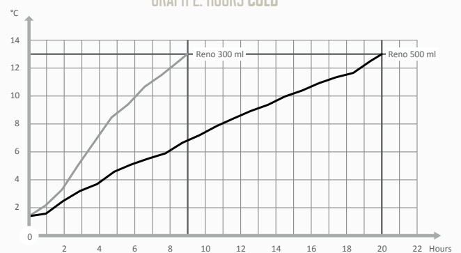
GRAPH 2: HOURS COLD
